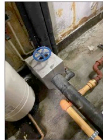
MAINS COLD WATER ISOLATION POINT.
